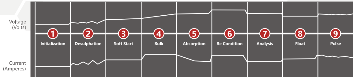
Automatic and High Frequency 9-Stage Charging Curve ■ For all smart charger apply on Gel and normal battery
