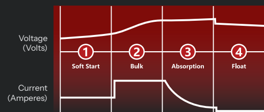
Automatic and High Frequency 4-Stage Charging Curve ■ For all smart charger, apply on Gel and normal battery
